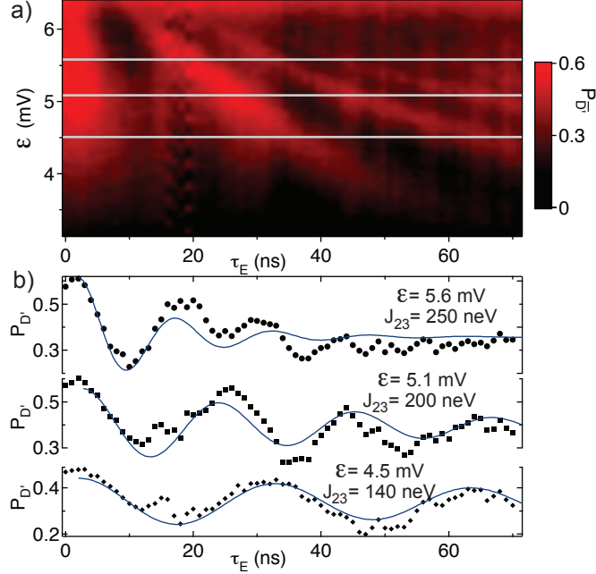
Figure 4.4: Coherent spin exchange a , Probability P_{\overline{D}'}_{S_z} to return to the initial |\overline{D}'_{S_z}\rangle state following an exchange pulse sequence, measured as a function of \epsilon during the exchange pulse and pulse duration \tau_E . Dark and bright regions respectively indicate odd and even numbers of complete spin exchanges. b , Points: Measured P_{\overline{D}'}_{S_z} as a function of \tau_E for values of \epsilon indicated by horizontal lines in a . Lines: Fits to exponentially damped phase-shifted cosines. The fitted exchange J_{23}(\epsilon) for each curve is shown.
